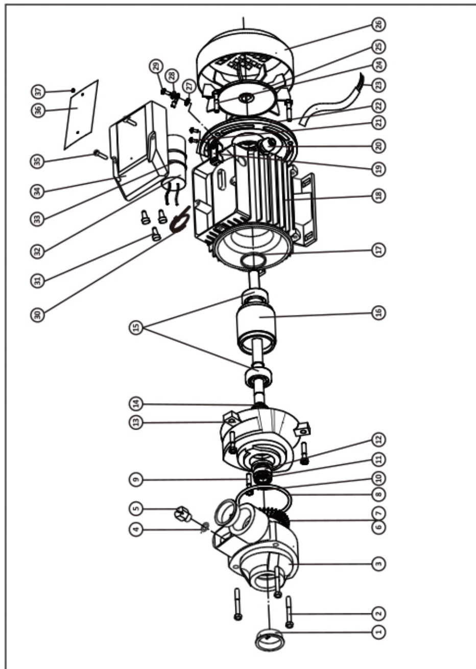
EXPLOSIVE VIEW OF WD020240370/WD020250750
